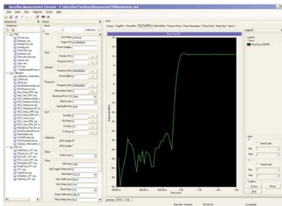
Fig 3. Transmit Mode Pulse Risetime
