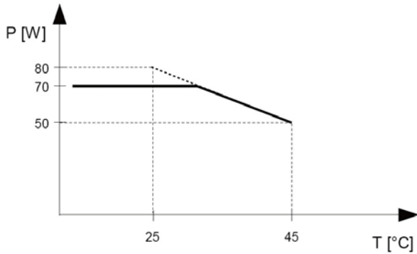
Maximum allowable continuous input power as a function of temperature
