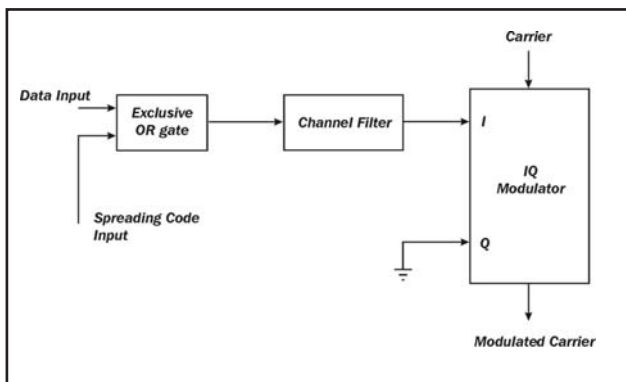
Figure 13 - BPSK Spread Spectrum with Channel Filter
