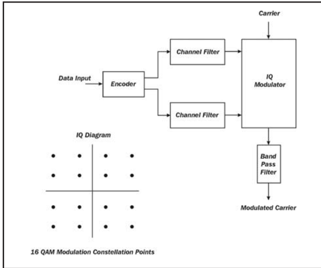
Figure 10 - QAM Modulation
