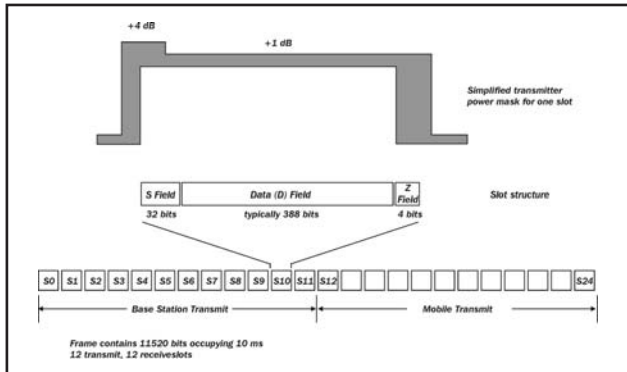
Figure 17 - DECT Data Structure
