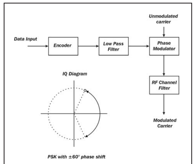
Figure 8 - Constant Amplitude PSK
