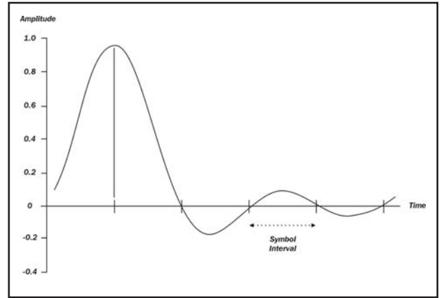
Figure 6a - Raised Cosine Filter (Impulse Response)
