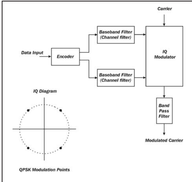
Figure 9 - PSK (Non Constant Amplitude)
