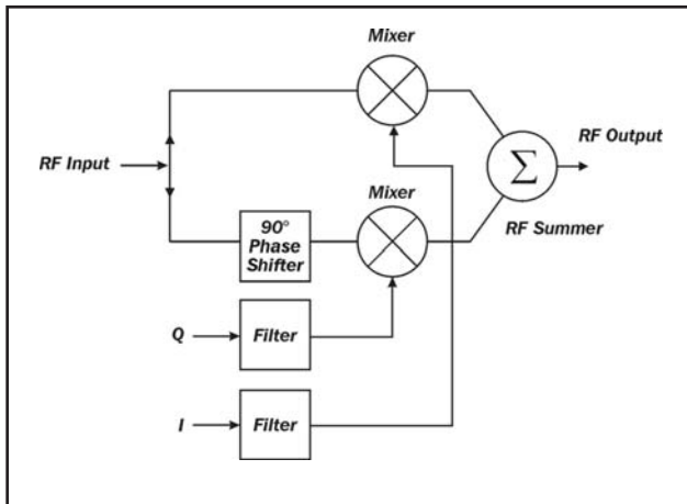
Figure 4 - IQ Modulator
