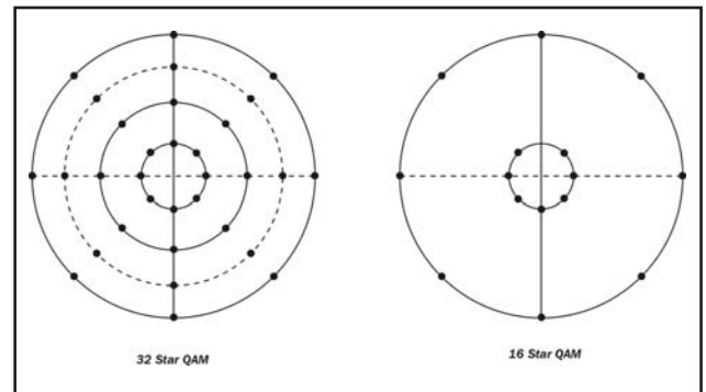
Figure 12 - Star QAM
