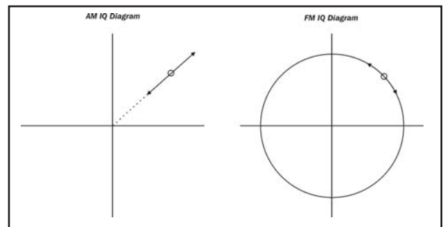
Figure 3 - AM and FM IQ Diagram
