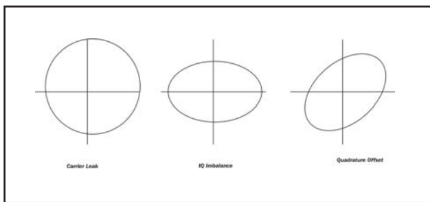
Figure 5 - Effect of IQ Modulator Errors
