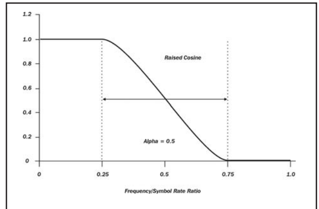
Figure 6b - Raised Cosine Frequency Response
