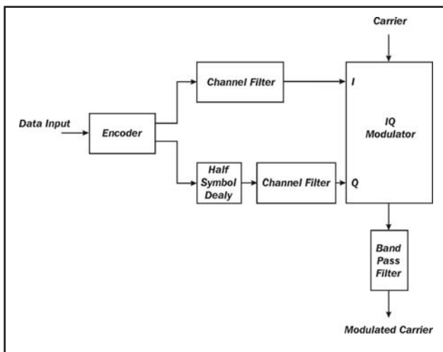
Figure 11 - Time Offset QAM
