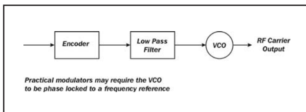
Figure 7 - FSK (Frequency Shift Keying)
