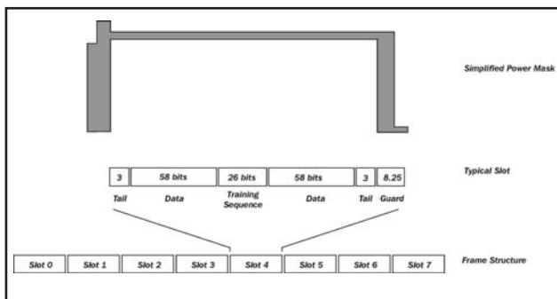
Figure 18 - GSM Structure
