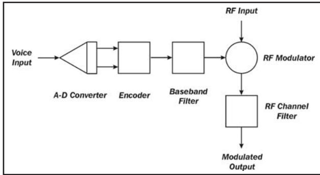
Figure 1 - Simplified Digital Modulator
