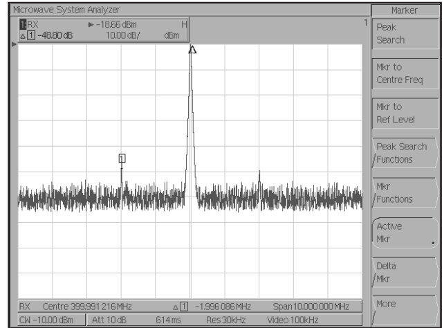
Fig. 18 Measurement of LO AM suppression.
