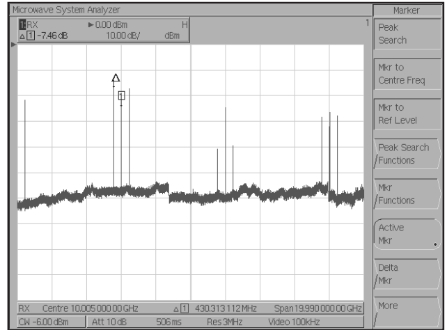
Fig. 5 IF Spectrum of mixer with no IF filtering.
