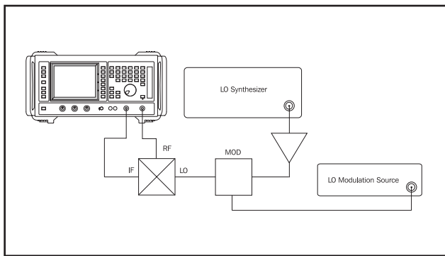
Fig. 17 Measurement of LO AM suppression
