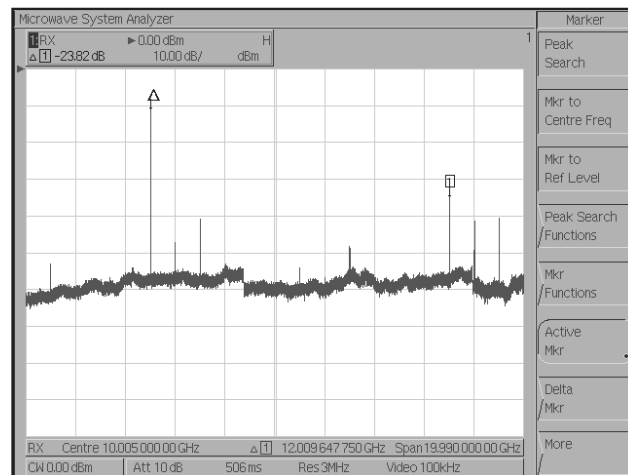
Fig. 2 Spectrum of IF signals
