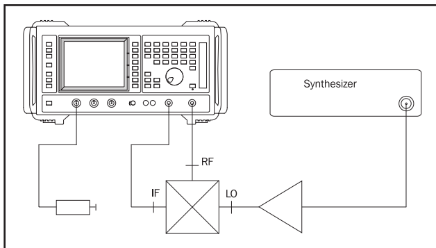
Fig. 1 Upconverter Test
