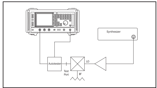
Fig. 7 Return Loss Measurements Using an Autotester.
