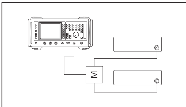
Fig. 11 Measurement of system two tone distortion
