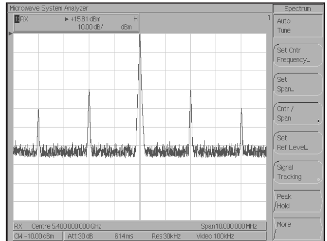
Fig. 15 Reference AM on Local Oscillator
