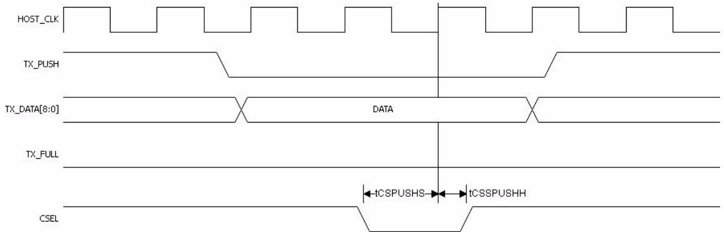
Figure 34. Transmit Port PUSH with Chip Select Transition
