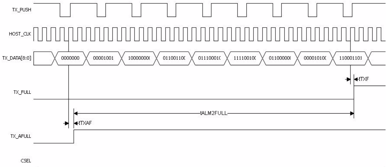
Figure 32. Transmit FIFO Almost Full Bag
