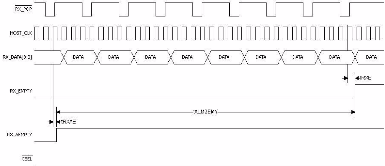
Figure 35. Receive FIFO Almost Empty Flag
