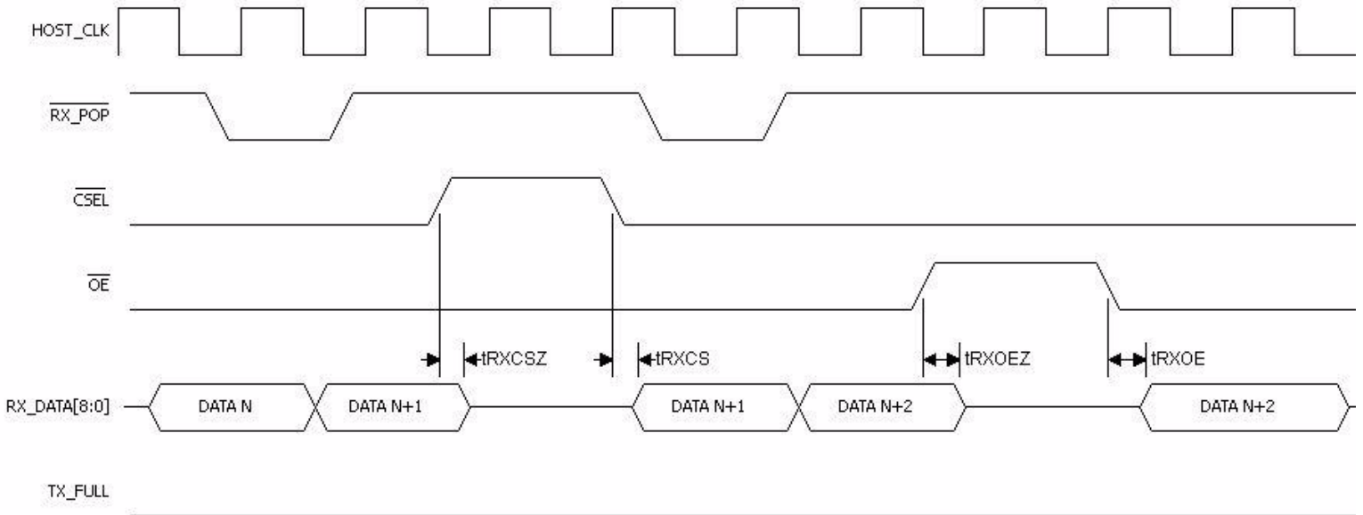
Figure 37. Control Inputs Timing Information
