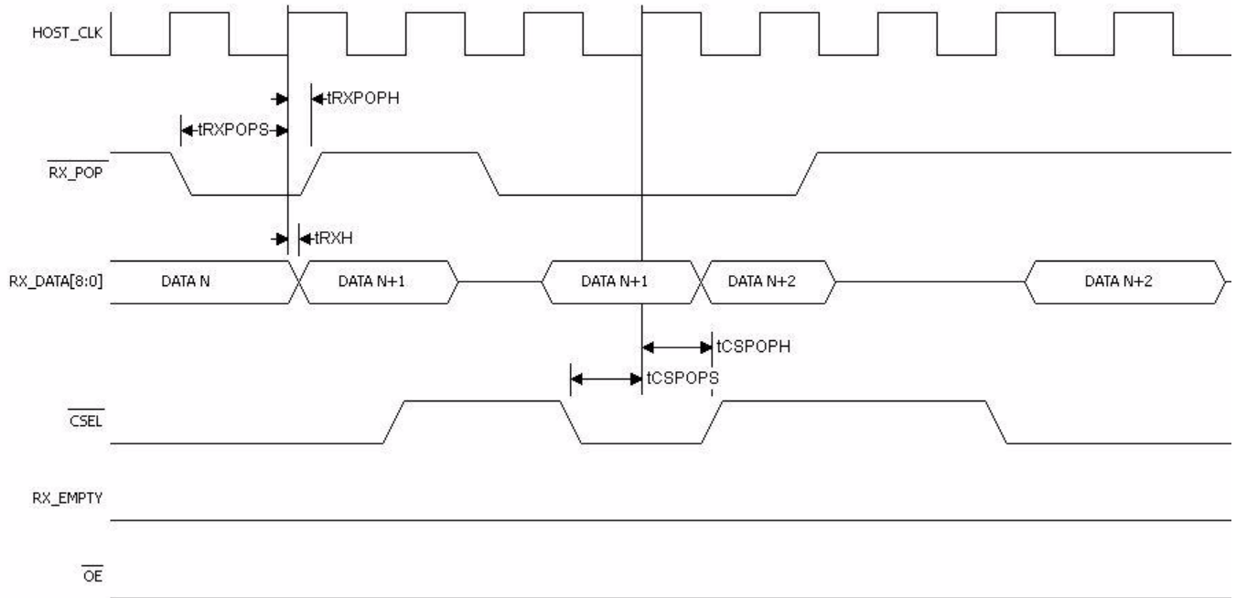
Figure 36. Receive Port POP System port read timing specification, reading data out of System Port FIFO
