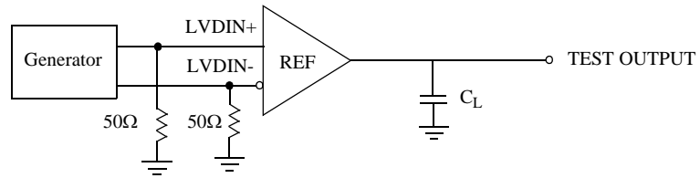
Figure 11. Receiver Propagation Delay and Transition Time Test Circuit or Equivalent Circuit
