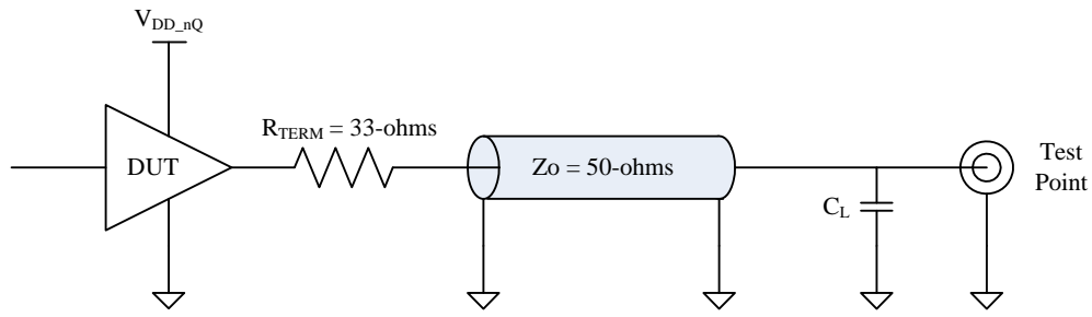
Figure 10A. Series Terminated LVC MOS/LVTTL Test Circuit
