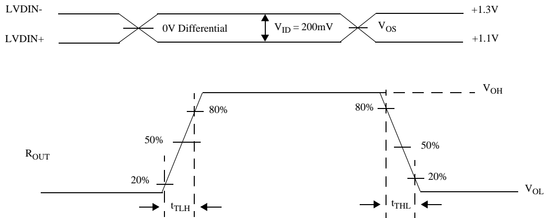
Figure 12. Receiver Transition Time Waveforms
