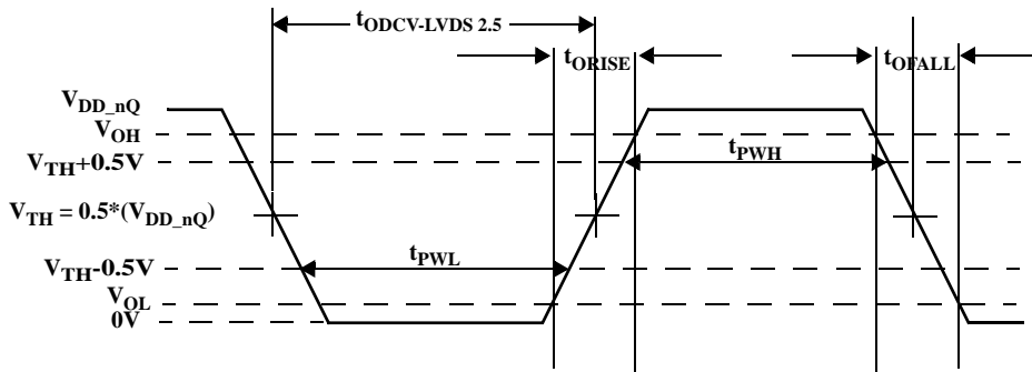
Figure 9B. +2.5V LVCMOS2.5/LVTTL Output Waveform
