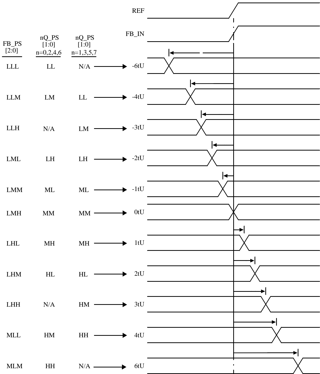
Figure 8b. Phase Select Time Unit Step Relationships
