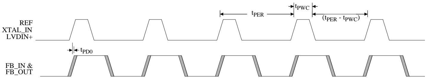
Figure 8a. Reference and Feedback Timing Diagrams
