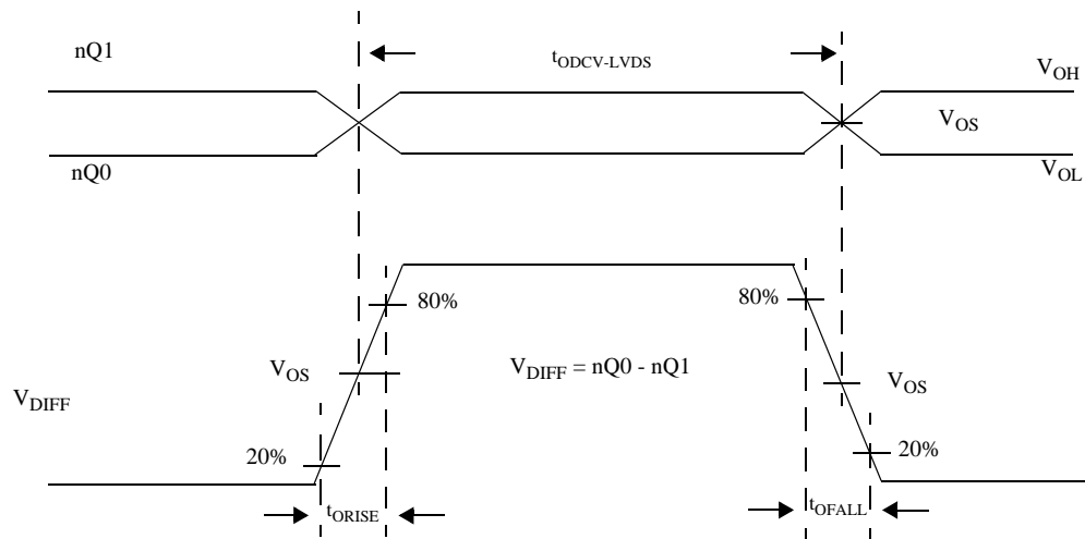
Figure 14. Driver Transition Time Waveforms
