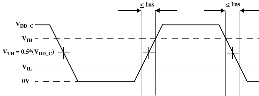
Figure 9C. LVCMOS3.3/LVTTL and XTAL_IN Input Test Waveform
