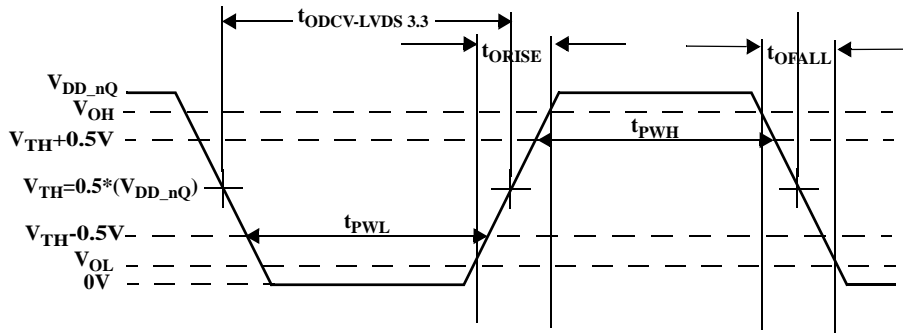
Figure 9A. +3.3V LVCMOS3.3/LVTTL Output Waveform
