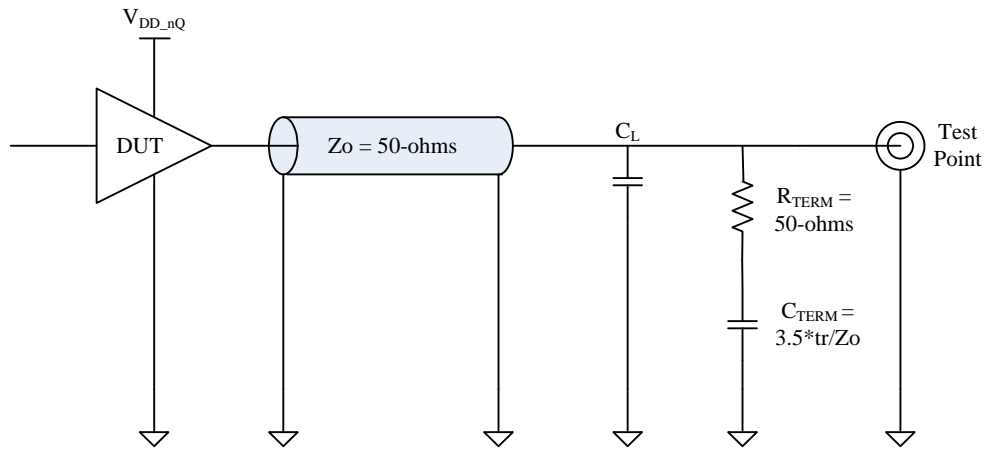
Figure 10C. AC Terminated LVC MOS/LVTTL Test Circuit
