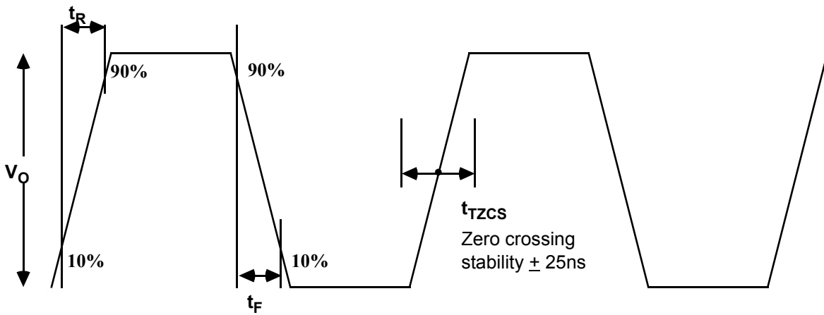
Figure 54. Transmitter Output Zero Crossing Stability, Rise Time, Fall Time ( t_{ZCS} , t_R , t_F )
