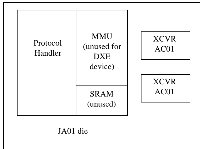
Figure 1. SμMMIT DXE Multi-Chip Module
