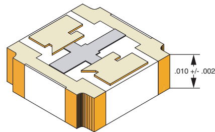
Front to Back Metallization in Four Places
