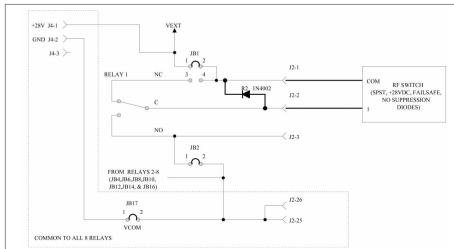
Figure 2. Typical SmartStep Relay Driver Setup
